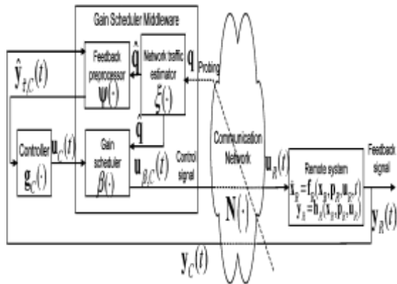
Fig. 5. Block diagram of the GSM module designed by Tipsuwan and Chow [27] for network delay compensation
